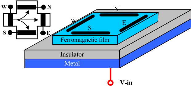
Fig. 8: Spin-wave switch.
