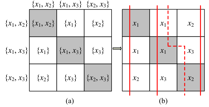
Fig. 12: Implementing f_T = x_1x_2 + x_1x_3 + x_2x_3 . (a): Lattice sites with corresponding sets. (b): Lattice sites with corresponding literals.
