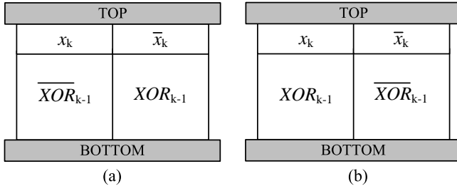
Fig. 16: (a): Implementation of XOR_k . (b): Implementation of \overline{XOR}_k .
