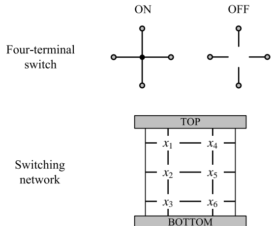
Fig. 2: Four-terminal switching network implementing the Boolean function x_1x_2x_3 + x_1x_2x_5x_6 + x_2x_3x_4x_5 + x_4x_5x_6 .
