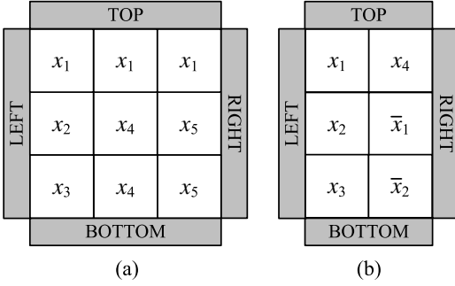
Fig. 19: Minimum-sized lattices (a): f_L = f_{T1} = x_1x_2x_3 + x_1x_4 + x_1x_5 . (b): f_L = f_{T2} = x_1x_2x_3 + \bar{x}_1\bar{x}_2x_4 + x_2x_3x_4 .
