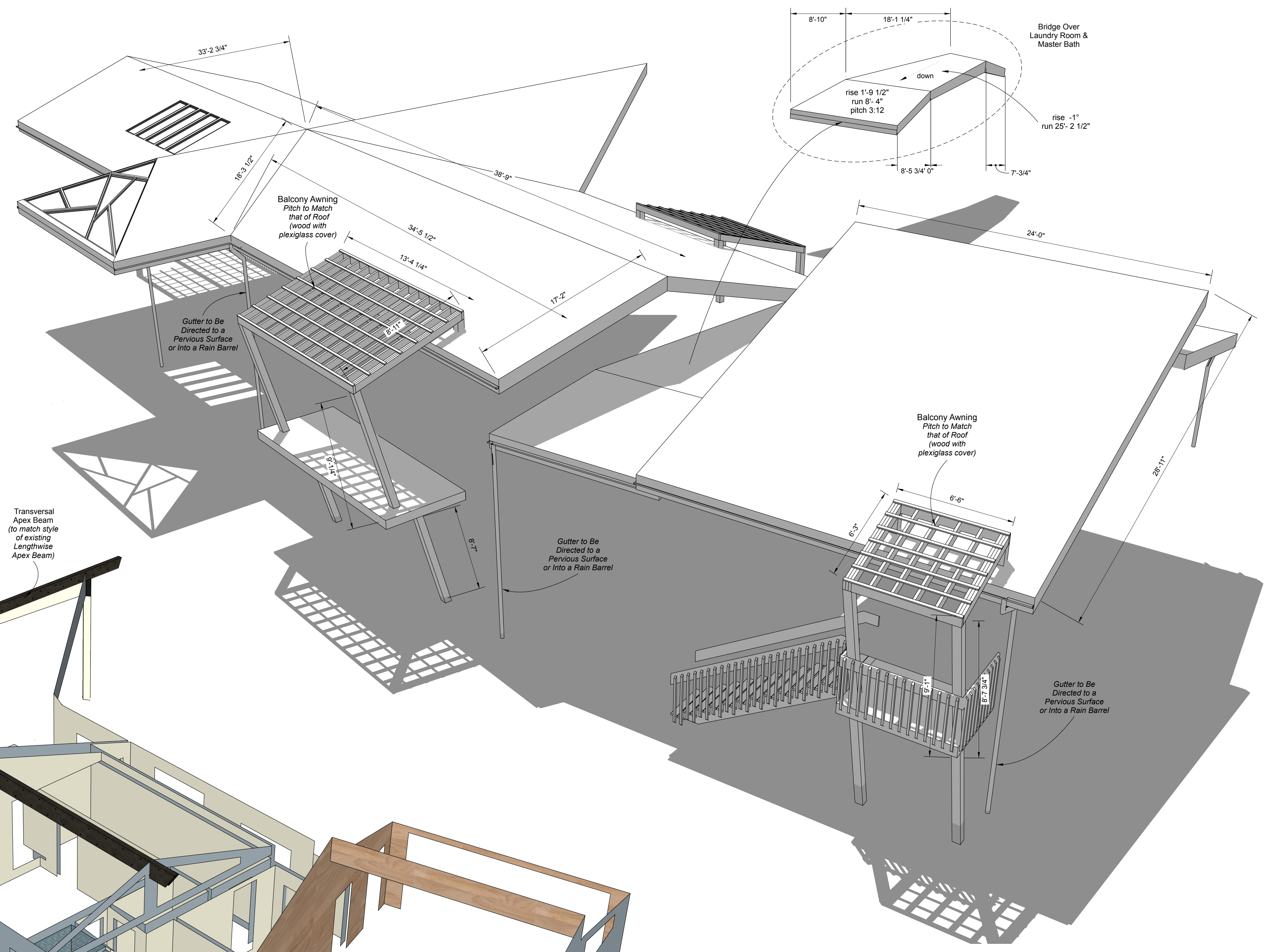
Roof Perspective From NE
