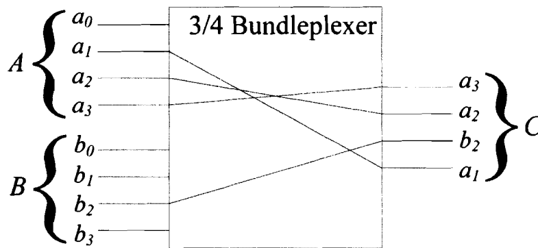
Figure 3. A bundleplexer with N = 4 and s = 3/4
