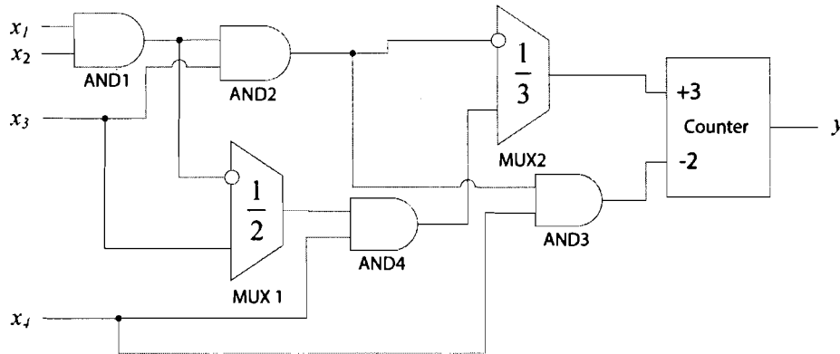
Figure 12. The stochastic circuit obtained from the UnitPosBMD in Figure 9 and the UnitNegBMD in Figure 7(b). The number on the counter indicates the amount that it increments or decrements the count for each 1 on the corresponding bundle. The output of the counter implements the function of the original *BMD in Figure 6.
