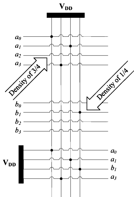
Figure 15. The nanowire crossbar architecture implementing a bundleplexer
