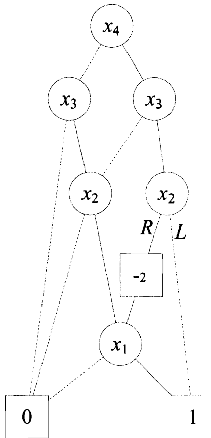
Figure 6. The *BMD for the circuit in Figure 5
