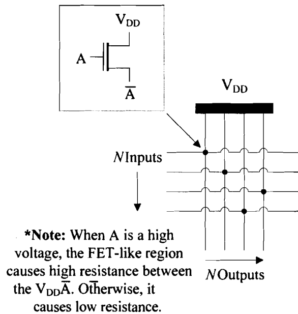
Figure 13. The nanowire crossbar architecture
